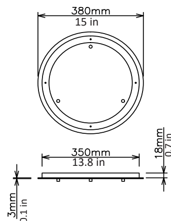
Ceiling plate
